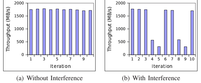
Figure 3. Experiments done on the Nancy site of Grid'5000 with 35 PVFS servers across an Infiniband network: (a) one instance of IOR runs on 336 cores and writes every 10 seconds; (b) another instance is started on 336 other cores and writes every 7 seconds (the figure represents the observed throughput of the first instance only).
