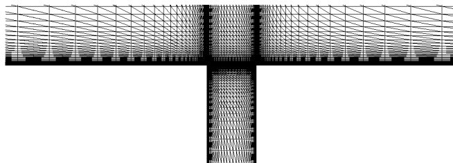
Figure 10: Mesh in the vicinity of the actuator, slot model.
