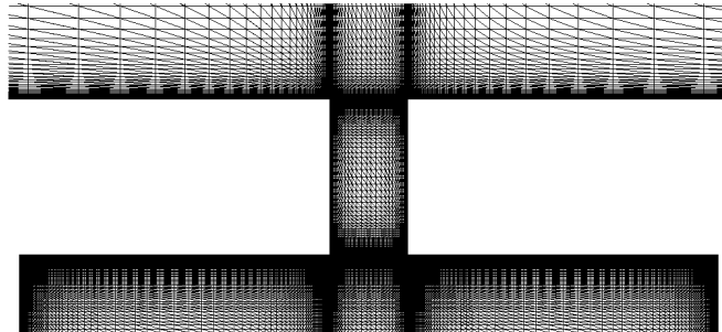
Figure 9: Mesh in the vicinity of the actuator, cavity model.
