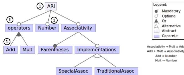
Fig. 3. VAM for the Expression Language
