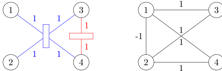
Figure 6: Hypergraph \mathbf{h}_5 from Example 4 and its reduced signed graph \tilde{\mathbf{h}}_5
