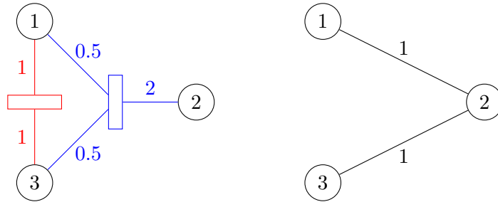
Figure 5: Hypergraph \mathbf{h}_4 from Example 4 and its reduced signed graph \tilde{\mathbf{h}}_4
