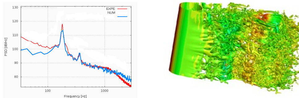
Figure 2: Left: Comparison of the energy spectrum between present simulations and experiments by Jenkins et al. Right: Isovorticity with pressure field (red= high pressure, blue= low pressure).
