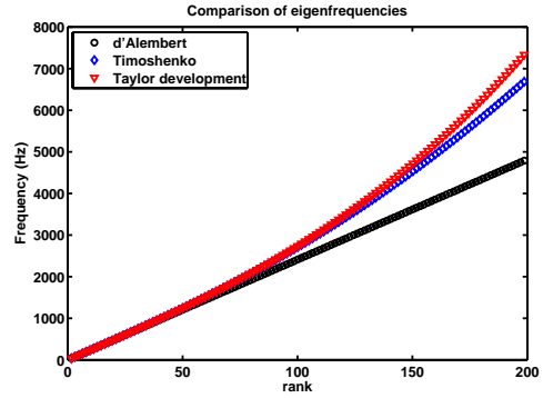
(b) Comparison between d'Alembert eigenfrequencies, Timoshenko and its Taylor expansion of formula (19).
