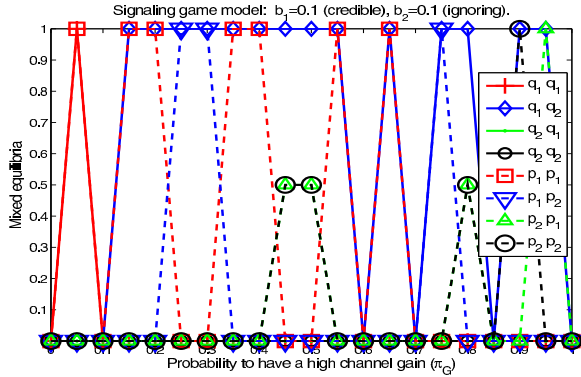
Figure 3: Mixed equilibria as function of \pi_G when player II does not believe in the received signal.
