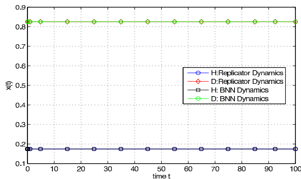
Fig. 7. Convergence of the Replicator Dynamics and the BNN dynamics to the ESS for a starting point \alpha_0 = \alpha^* = 0.825 . Here we converge to the mixed ESS \alpha^* .
