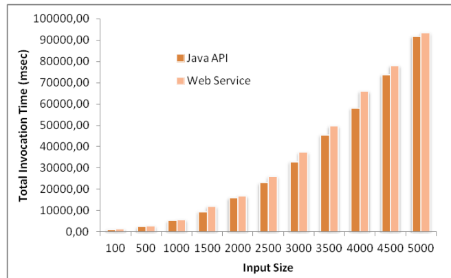
Figure 4.19: Total execution time for the invocation of the AbstractWeatherForecastService
