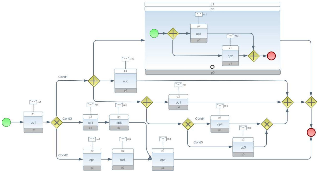
Figure 4.7: BPMN2 choreography diagram example
