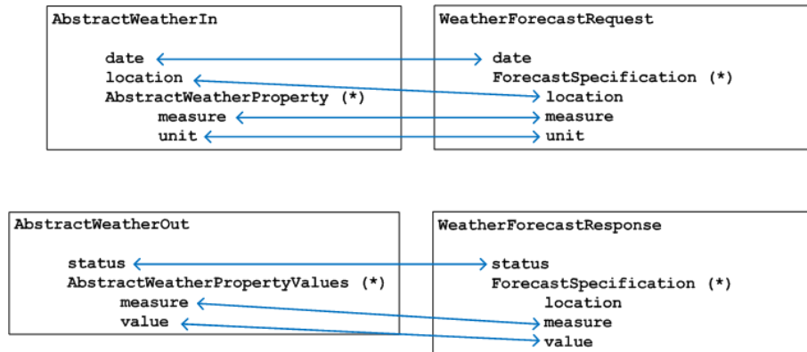
Figure 2.5: Operation mappings for the weather service abstraction.
