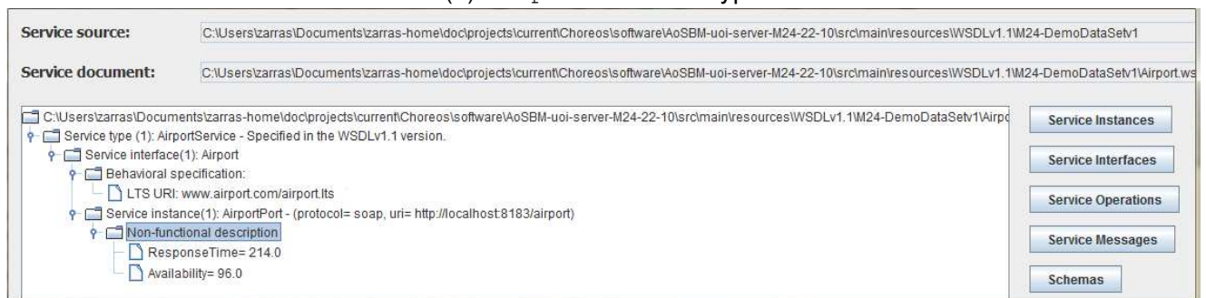
(b) AirportService instance
