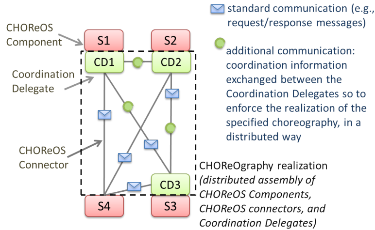
Figure 4.1: CHOReOS choreography
