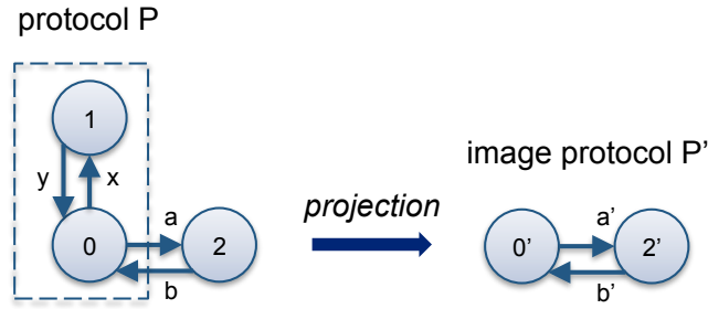
Figure 3.23: Protocol projection
