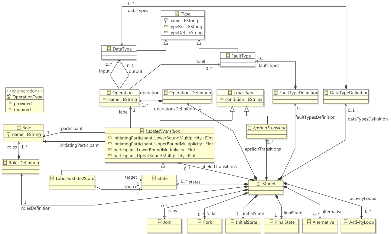
Figure 4.3: CLTS metamodel
