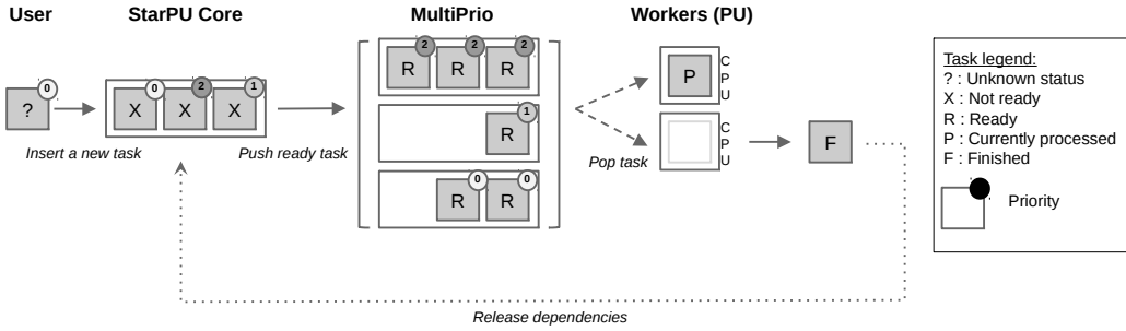
Fig. 3.9: Priority scheduler
