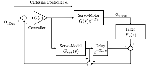
Fig. 10: Scheme of the Smith predictor for \alpha_i including the controller C(s) , the servo motor G(s)e^{-Ts} , the model of the servo motor G_{est}(s)e^{-T_{est}s} , and the Butterworth filter B_2(s)
