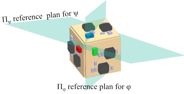
Fig. 7. Definition of the second reference plane \Pi_\psi in relation with the first reference plane \Pi_\varphi . Note that the plane \Pi_\psi is orthogonal to the plane \Pi_\varphi .
