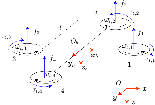
Fig. 2. Thrusters related variables
