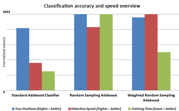
Figure 6: Classifier comparison
