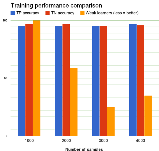
Figure 3: Random sampling training is performed with subsets of 1k, 2k, 3k and 4k size. The 3k subset (10.7% of parent set) reveals adequate discrimination and requires a low number of weak learners
