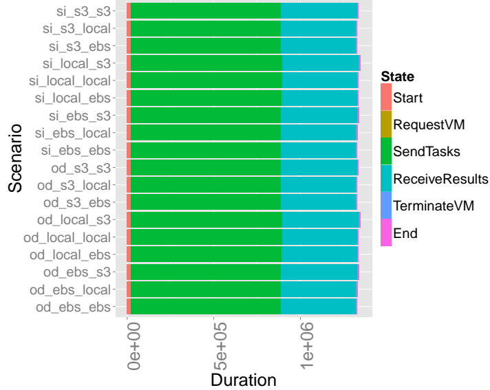
Figure 8: Makespan of SimpleBoT for each scenario.
