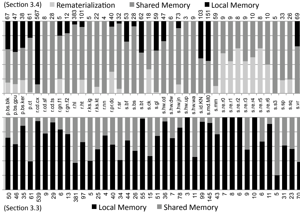
Fig. 24. Target location of instructions used to load the variables spilled by AffRA with eight registers and DivRA with nine. The numbers give the total quantity of load instructions.
