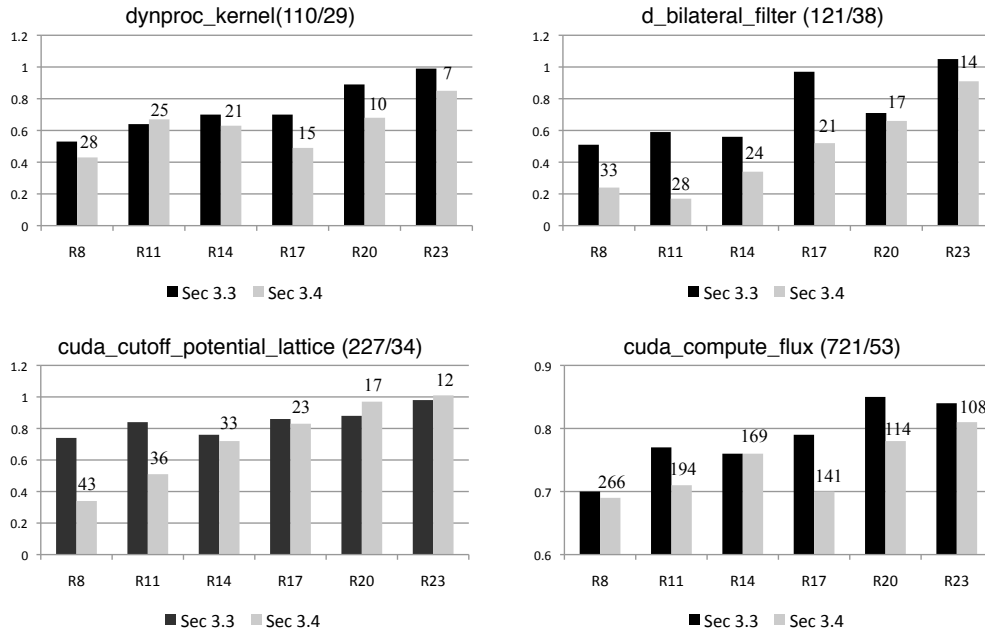
Fig. 28. Runtime of code produced by the different register allocators versus the number of available registers. Bars are normalized by the runtime of code produced by Ocelot’s linear scan. Values above bars show number of variables spilled by AffRA. Values next to kernel names give number of PTX instructions in the program, and maximum register pressure. The shorter the bar, the faster the code.
