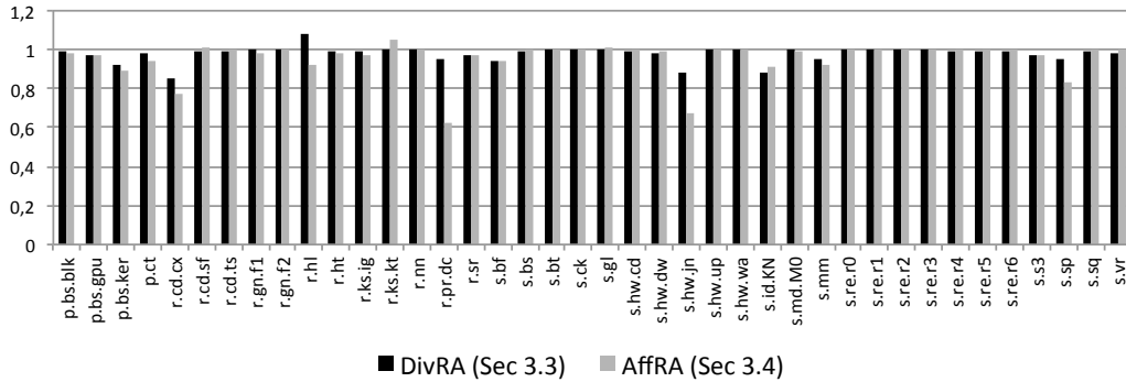
Fig. 27. Relative speedup obtained by different register allocators in a setup with 21 registers available for each thread. Like in Figure 23, bars are normalized to the time given by Ocelot’s linear scan register allocator. The shorter the bar, the faster the kernel.
