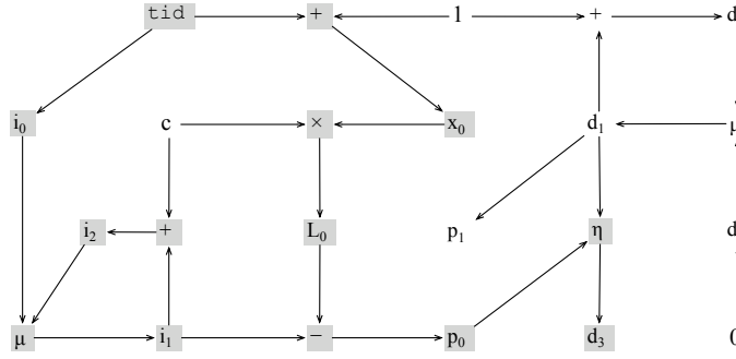
Fig. 11. The dependence graph created for the program in Figure 9. We only show the program slice [Weiser 1981] that creates variables p_1 and d_3 . Divergent variables are colored gray.
