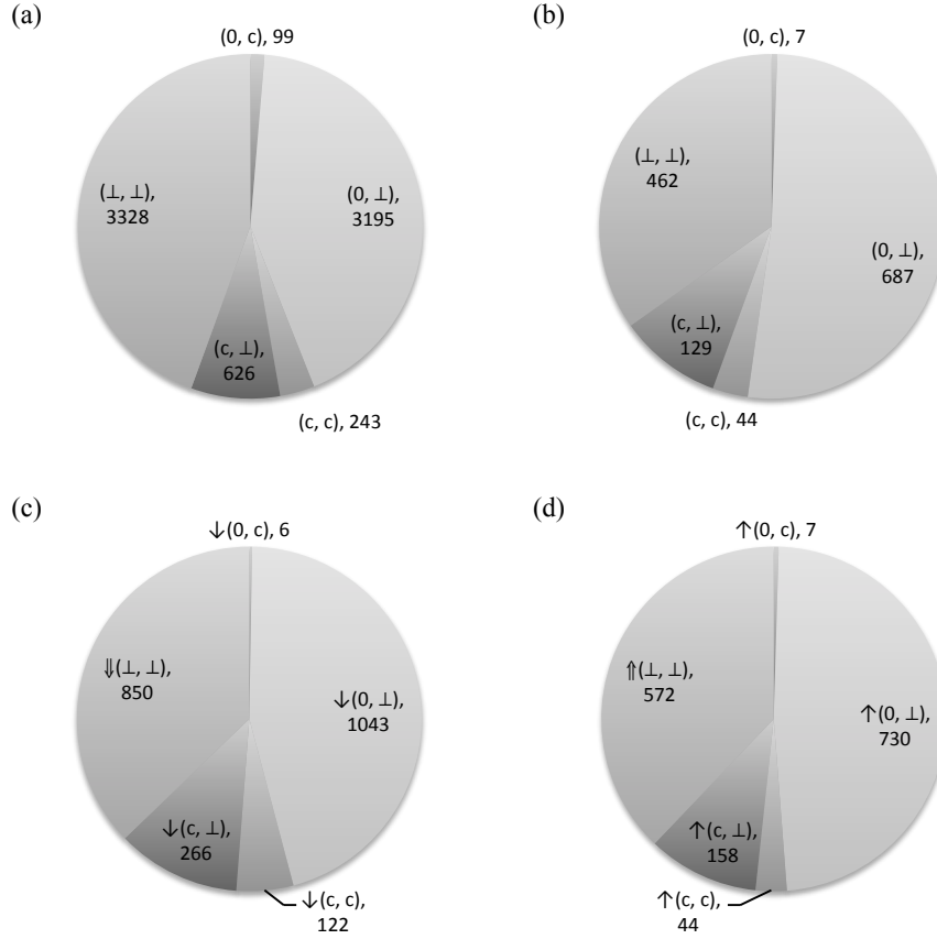
Fig. 26. (a) Distribution of abstract states among the variables in our test suite of 40 kernels. (b) Abstract state of the variables spilled by AffRA with eight registers. (c) Type of instructions used to load or rematerialize spilled values. (d) Type of instructions used to store spilled values.
