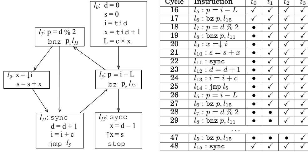
Fig. 8. (Left) Example of a \mu -SIMD program. (Right) Snapshot of the execution trace of the \mu -SIMD program on the left. If a thread t executes an instruction at a cycle j , we mark the entry (t, j) with the symbol ✓. Otherwise, we mark it with the symbol •.
