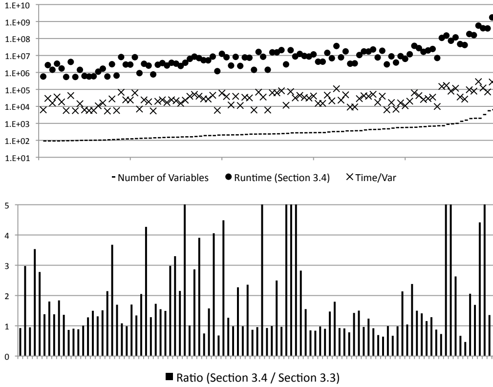
Fig. 21. (Top) Time, in CPU cycles, to run the divergent analyses compared with the number of variables per kernel in GSA-form. Points in the X-axis are kernels, sorted by the number of variables they contain. (Bottom) Comparison between times to run our two divergence analyses. Each bar gives time of affine analysis over time of simple analysis. We have cropped bars that exceed a slowdown of 5x. We report time of analyses only, excluding other compilation phases.
