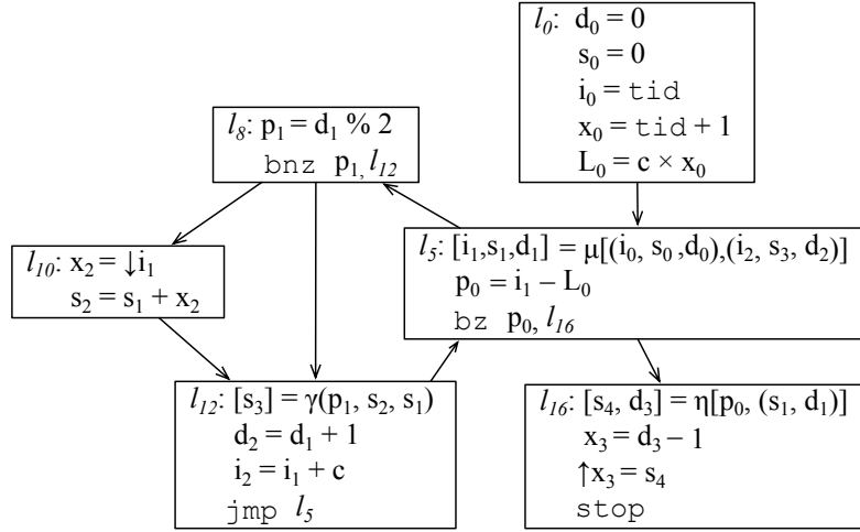
Fig. 9. The program from Figure 8 converted into GSA form.
