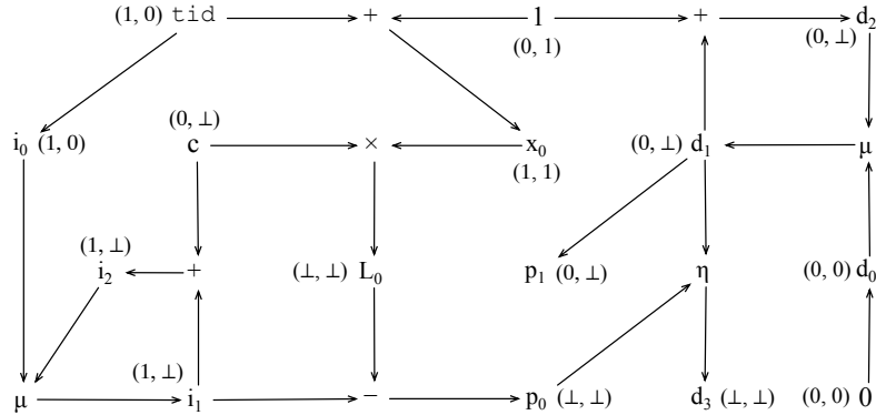
Fig. 14. Results of the divergence analysis with affine constraints for the program slice seen in Figure 11.
