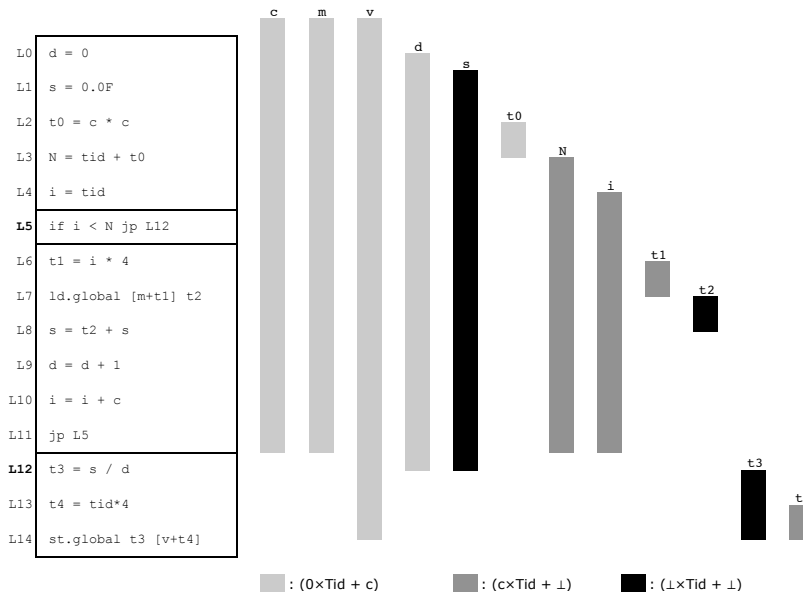
Fig. 16. The register allocation problem for the kernel avgSquare in Figure 1.
