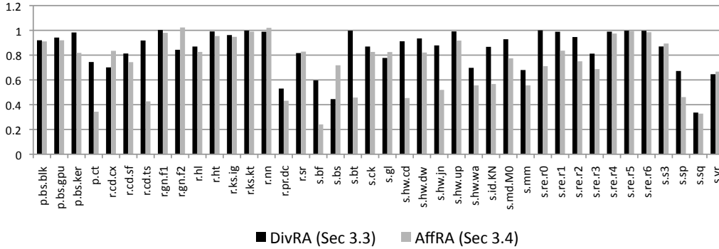
Fig. 23. Relative kernel execution time with different register allocators. Every bar is normalized to the time given by Ocelot's linear scan register allocator. The shorter the bar, the faster the kernel.
