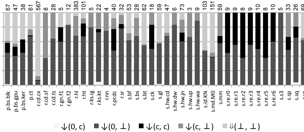
Fig. 25. Type of reconstruction code inserted by AffRA with polynomials of degree one. Values above bars give number of uses of spilled variables.
