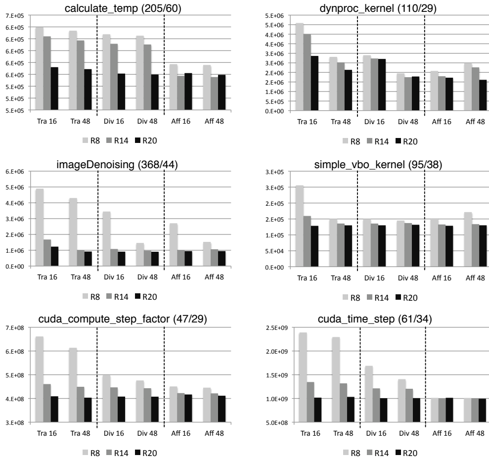
Fig. 29. Impact of the cache configuration on the runtime of six benchmarks. Bars shows absolute times, in CPU ticks. Tra is the traditional (divergence oblivious) allocator. We use Div for DivRA, and Aff for AffRA. We write 16 to denote a 16KB L1 cache, and 48 to denote a 48KB L1 cache.
