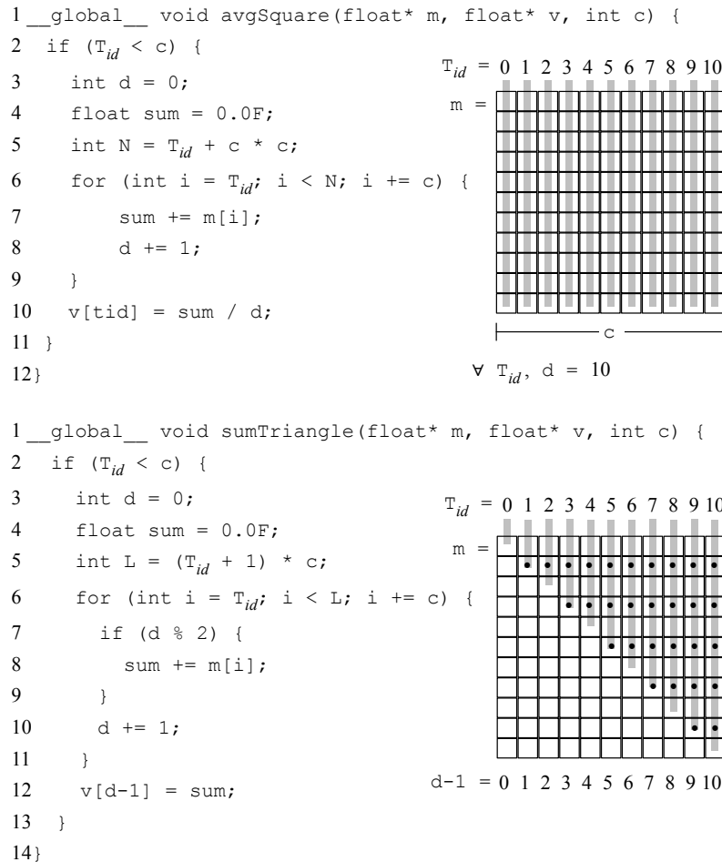
Fig. 1. Two kernels written in C for CUDA. The gray lines in the right show the parts of matrix m processed by each thread. Following usual coding practices we represent the matrix in a linear format. Dots mark the cells that add up to the sum in line 8 of sumTriangle .
