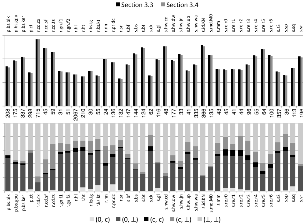
Fig. 22. (Top) Percentage of divergent variables (0-100%) reported by the simple divergence analysis of Section 3.3, and the divergence analysis with affine constraints of Section 3.4. (Bottom) Abstract states that the divergence analysis with affine constraints of Section 3.4 finds for the program variables. Values between charts give number of variables in each kernel in GSA form.
