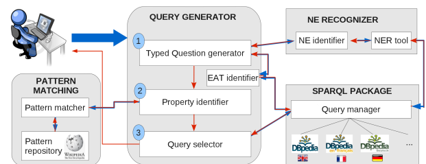
Figure 4. QAKiS workflow
