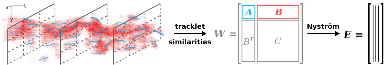
Fig. 3: Illustration of the Nyström approximation. We first sample n \ll N tracklets by randomly choosing p points in each cell of a regular spatio-temporal grid. We then compute the similarity between the selected tracklets (in blue), yielding matrix A , as well as with all other N - n points (in red), yielding matrix B . The Nyström method allows to efficiently compute a spectral embedding E from the approximate leading eigenvectors \hat{U} of the large N \times N matrix W of all similarities using only the small n \times N slice of it, composed of blocks A and B .
