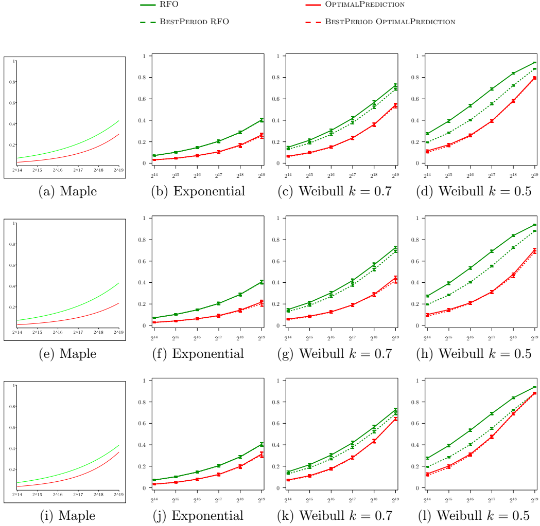
Figure B.10: Waste (y-axis) for the different heuristics as a function of the platform size (x-axis), with p = 0.82 , r = 0.85 , C_p = C (first row), C_p = 0.1C (second row), or C_p = 2C (third row) and with a trace of false predictions parametrized by a uniform distribution.
