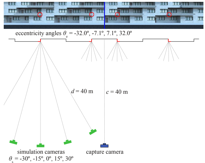
Figure 5: Wide-angle image (cropped) from the capture camera (optical axis in blue, corners in red), and stimulus creation parameters.
