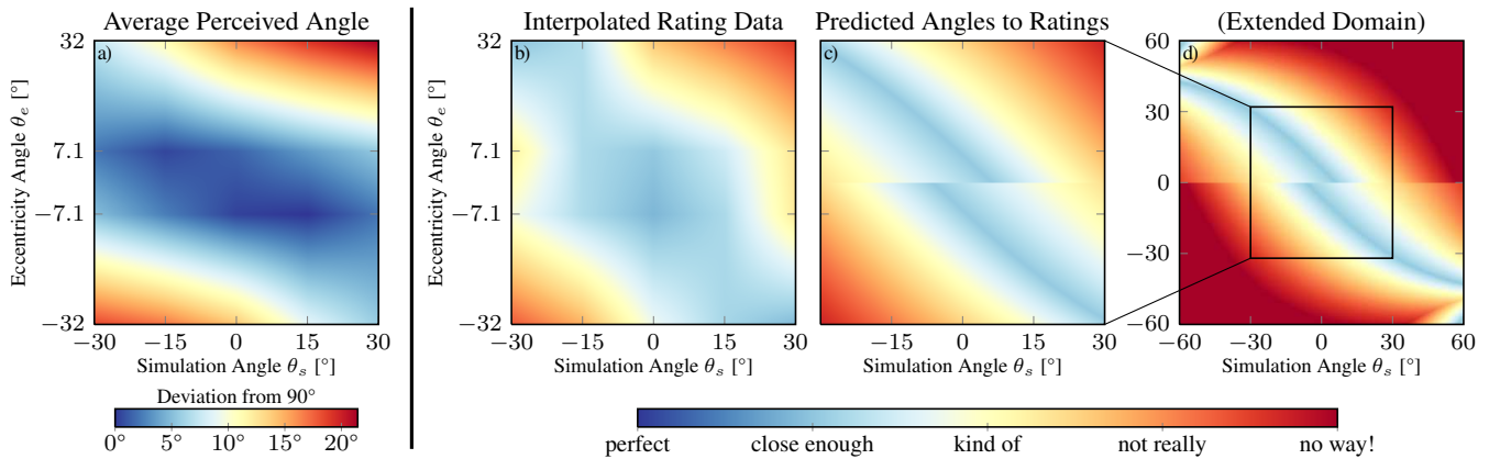
Figure 12: (a) The deviation of averaged perceived angles (Experiment 1) from 90^\circ has a similar pattern as (b), the interpolated medians of ratings from Experiment 2 (both linearly interpolated). (c) Perceived angles predicted by Eq. 19 mapped to ratings using Eq. 20, and (d) the same for an extended domain.
