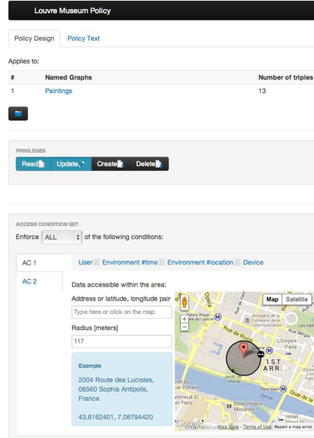
Fig. 2: The Shi3ld user interface.
