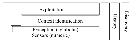
Figure 1: Model for context in pervasive computing. Data coming from sensors are aggregated and elaborated into the context used by applications (from[7]). This paper does not consider the orthogonal aspects (discovery, history and security).
