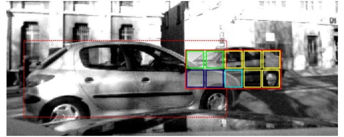
Fig. 9. Different categories of the patches of a detection. The patches can be considered as either (yellow) visible, (cyan) occluded considering stereo depth information, (green) occluded considering another detection nearer to the sensor, or (blue) occluded considering both of the above.
