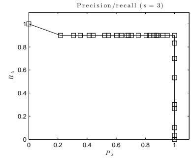
Fig. 6: Precision/recall graph for 3D problem ( w = 10 )
