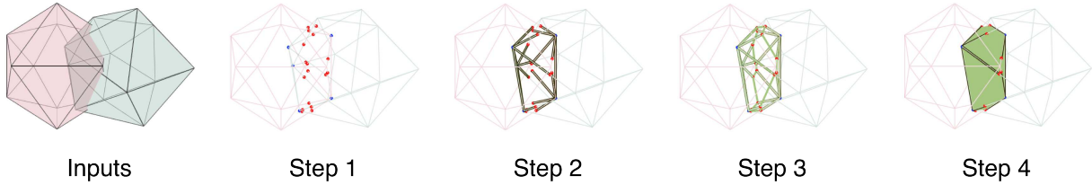
Figure 3: Steps of the proposed algorithm. Step 1: Intersection vertices, at the locus of edge to face intersections. Step 2: Restricted edges, initial edges restricted to portions inside the other polyhedron. Step 3: intersected edges materializing surface-to-surface intersections of the polyhedra. Step 4: Face identification by oriented walkthrough of the connected edges.
