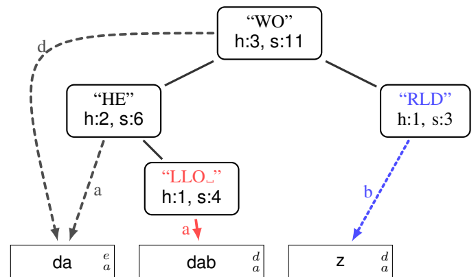
Figure 3: Tree-based implementation data structures
