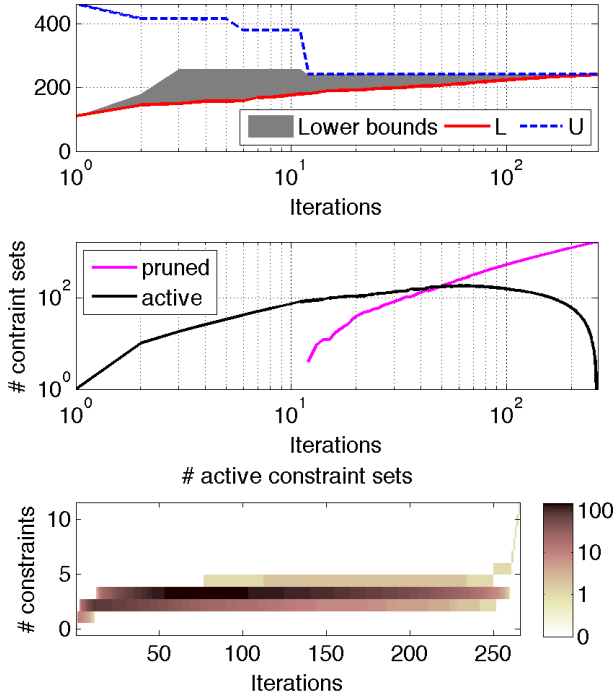
Fig. 2. Typical behavior of the proposed algorithm along the iterations. Top: lowest lower bound L , lowest upper bound U and area representing the range of all active lower bounds in \mathcal{A} . Middle: number of active and pruned constraint sets in \mathcal{A} . Bottom: histogram of the number of constraints among elements in \mathcal{A} .
