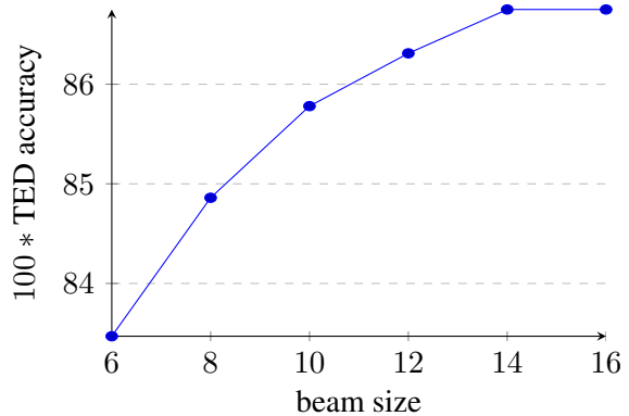
Figure 4: Score on Hebrew lattices w.r.t. beam size
