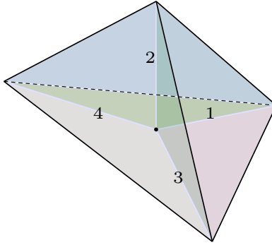
FIGURE 5. Clough–Tocher split.
