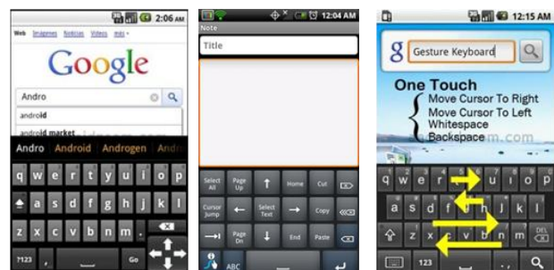
Figure 1. Solutions for caret movement: arrow keys (left - Arrows Keyboard [2], middle - Swipe [17]) and gestures (right - Gesture Keyboard [9]).
