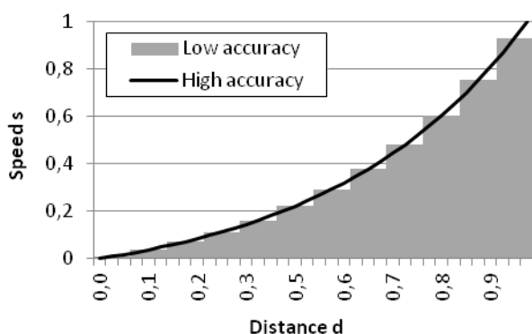
Figure 7. The exponential (3) mapping with different accuracies.
