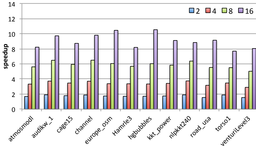
(a) SCALESK
