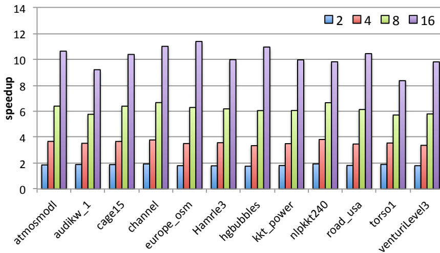
(b) ONESIDEDMATCH
