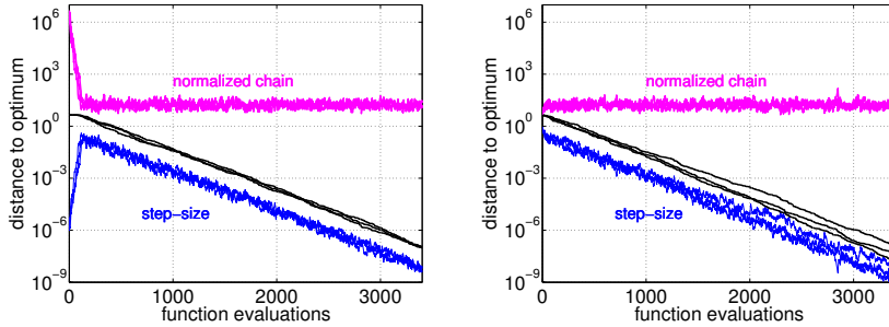
FIG. 5.1. Convergence simulations of the (1+1)-ES with generalized one-fifth success rule on spherical functions f(\mathbf{x}) = g(\|\mathbf{x}\|) for g \in \mathcal{M} in dimension n = 20 (parameters \gamma = \exp(1/3) and q = 4 ). Each plot is in log scale and depicts in black the distance to optimum, i.e., \|\mathbf{X}_t\| , in blue the respective step-size \sigma_t and in magenta the norm of the normalized chain \|\mathbf{Z}_t\| . The x-axis is the number of function evaluations corresponding to the iteration index t . On the left the simulation is voluntarily started with a too small step-size equal to \sigma_0 = 10^{-6} to illustrate the adaptivity ability of the algorithm. On the right, the initial step-size equals 1.
