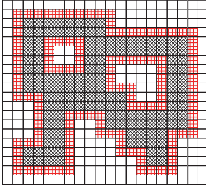
Figure 4: The cells of a domain \Omega are diagonally hatched. The domain \Omega_1^\epsilon is the whole shaded area and might be formed by cells of T'' .
