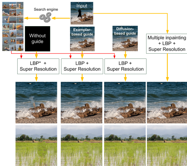
Fig. 13. Extension of the proposed approach. From a set of similar images, an inpainting is performed on a low-resolution version of the input picture. The LBP uses a set of similar images (21 images here (top-left)) and a guide (if any). The SR is applied to recover the details of the missing pixels. Different guides (exemplar-based or diffusion-based inpainting) can be used to drive the LBP. (*) (in the first box on the left) means that the term V_g of equation (13) is null. Bottom-up line gives other results.
