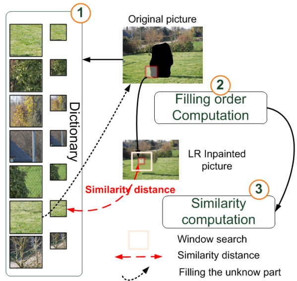
Fig. 6. Flowchart of the super-resolution algorithm. The missing parts of the red block are filled in by the best candidate stemming either from the dictionary or from the local neighbourhood. The top image represents the original image with the missing areas whereas the bottom one is the result of the low-resolution inpainting.
