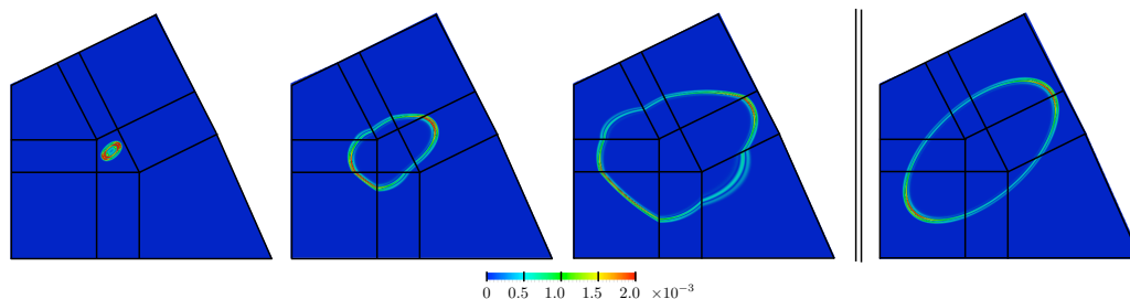
Figure 8. Left: snapshots at time t = 3.2, 16, 28.8 of the absolute value of the solution computed with \tau_0 = 0 and L = 40 . Right: snapshot at t = 20 of the reference solution u_{ref} computed in a large domain L = 40 .
