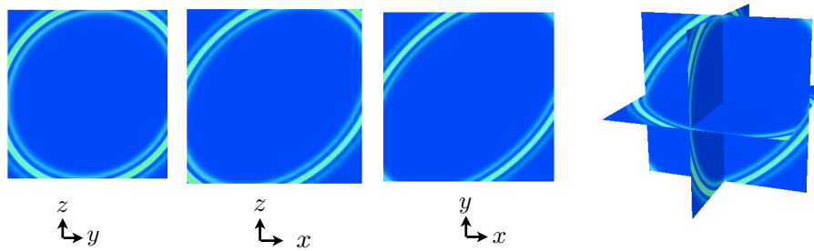
Figure 13. Snapshots at time t = 10.79 (color scale compressed 1000 times) of the absolute value of the solution.
