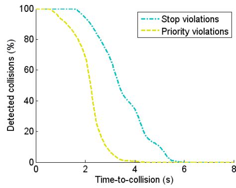
Figure 7: Comparison of the performance for priority violations scenarios and stop violations scenarios.
