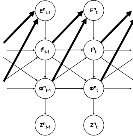
Figure 2: Graphical representation of the proposed MSSM. Bold arrows represent multi-vehicle dependencies, i.e. the influences of the other vehicles on vehicle n .
