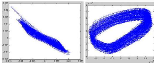
Figure 10. Observed change of polarization on a piano string. The photodetectors form an angle of 45^\circ with the vertical plane. The left figure shows the vertical motion of the string just after the blow, while the right figure shows its horizontal motion after several seconds.
