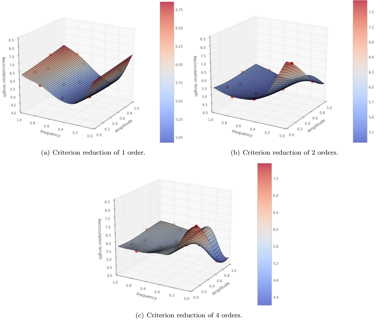
Figure 9. Non linearities convergence criterion effect on the recirculation length with k - \omega -ne-easm turbulence closure, a fine grid and a 256 time steps per period.
