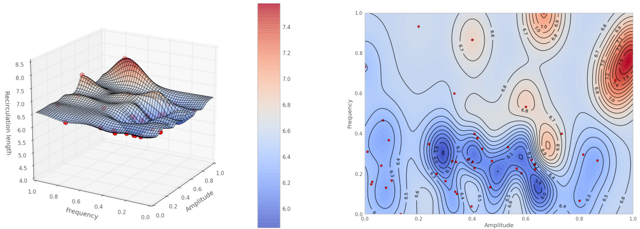
Figure 11. Final interpolating meta-model for the optimization of the recirculation length. The solver is the compressible one with a Spalart-Allmaras closure. For the optimization, we used the lower bound merit function and the final database contains 42 points in total.
