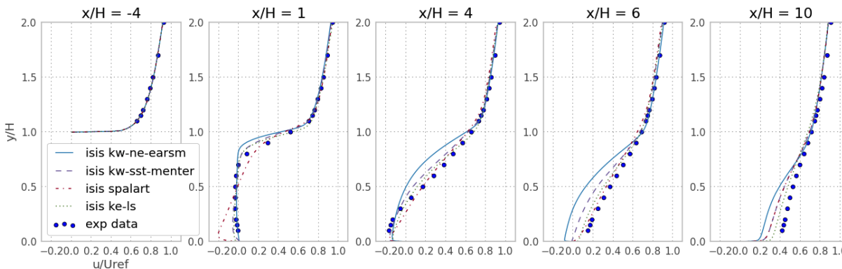
Figure 4. Initial velocity profiles at x = -4, x = 1, x = 4, x = 6 and x = 10 for different turbulence closures for the flow over the backward facing step without control.
