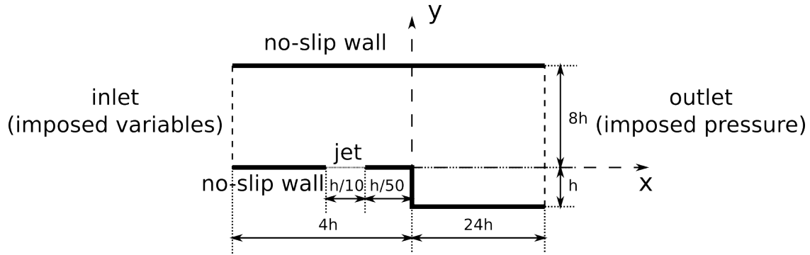
Figure 2. Backward-facing step configuration.
