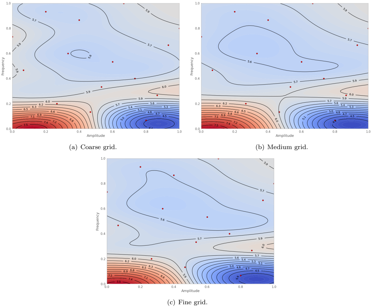
Figure 7. Grid refinement effect on the recirculation length with kw-ne-easm turbulence closure and 256 time steps by periods.
