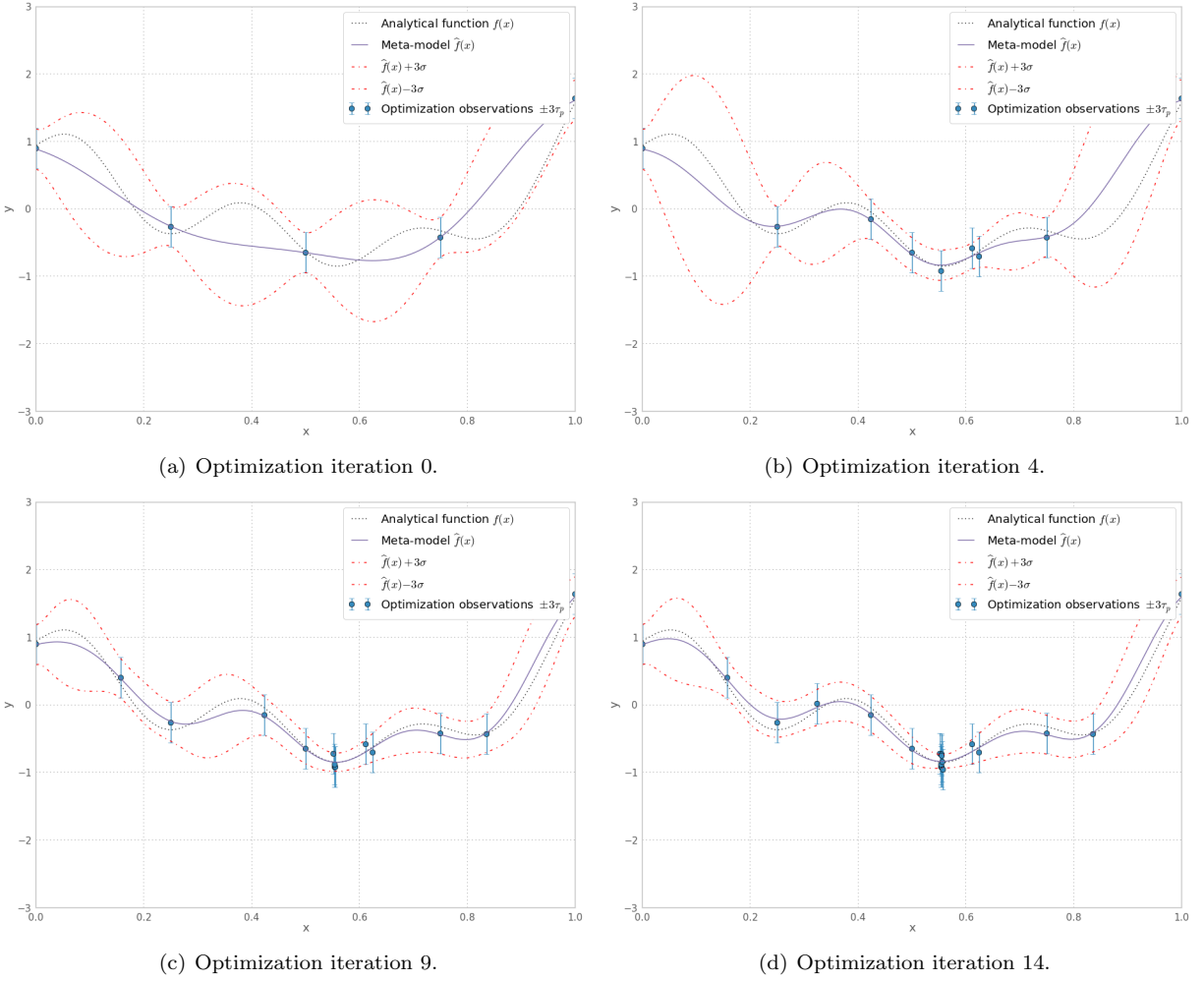
Figure 13. Optimization with the expected improvement of a 1D function using \tau_p = 0.1 and non-interpolating meta-model, with an observation uncertainty standard deviation set to \tau_i = 0.1 .
