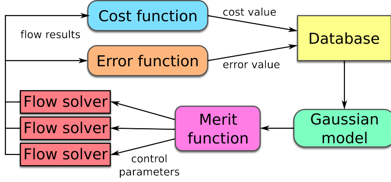
Figure 1. Efficient Global Optimization loop.
