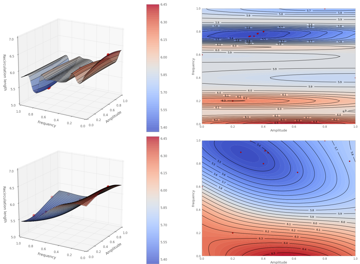
Figure 16. Comparison of meta-models after five optimization iterations of jet amplitude and frequency parameters using PI and AEI. The k-\omega -SST Menter model, 128 time steps per period and a reduction of non linear residuals of 3 orders is used. The PI (top), AEI (bottom) merit functions are used.
