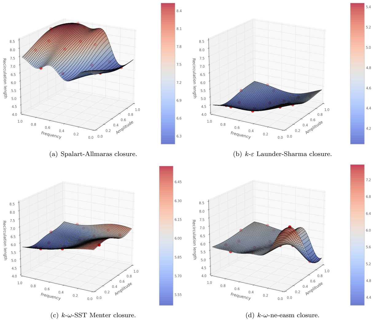
Figure 5. Influence of turbulence closures on the recirculation length.
