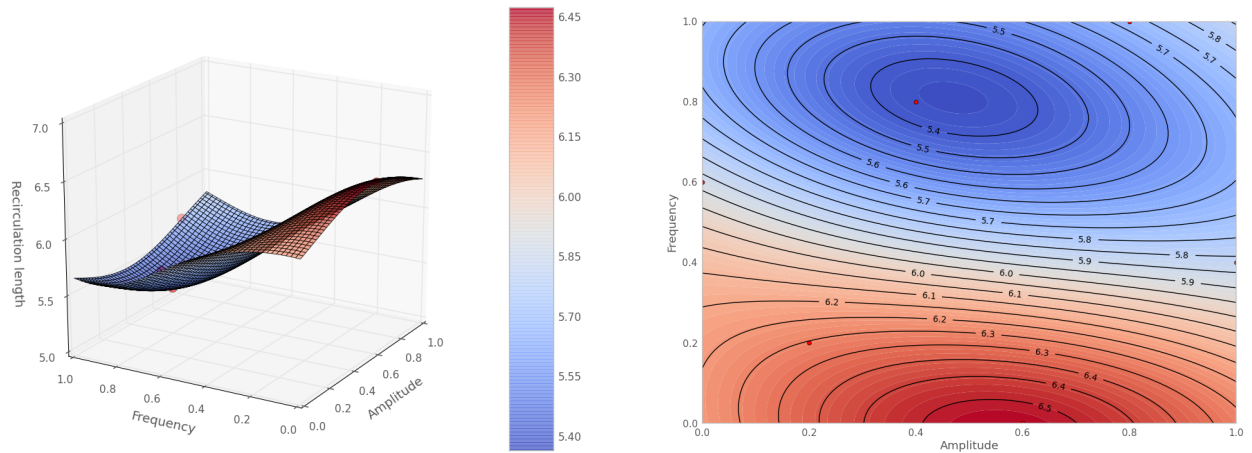
Figure 15. Initial database generated for the optimization of jet amplitude and frequency. The k-\omega -SST Menter model, 128 time steps per period and a reduction of non linear residuals of 3 orders is used.
