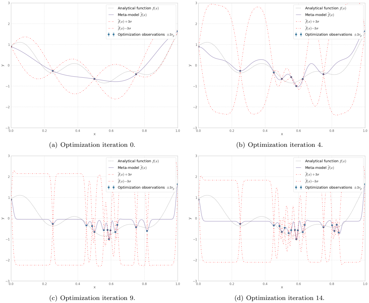
Figure 12. Optimization with the expected improvement of a 1D function using \tau_p = 0.1 and an interpolating meta-model.
