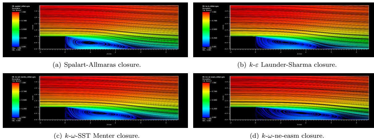
Figure 3. Comparison of velocity streamlines for different turbulence closures for the flow over the backward facing step without control.
