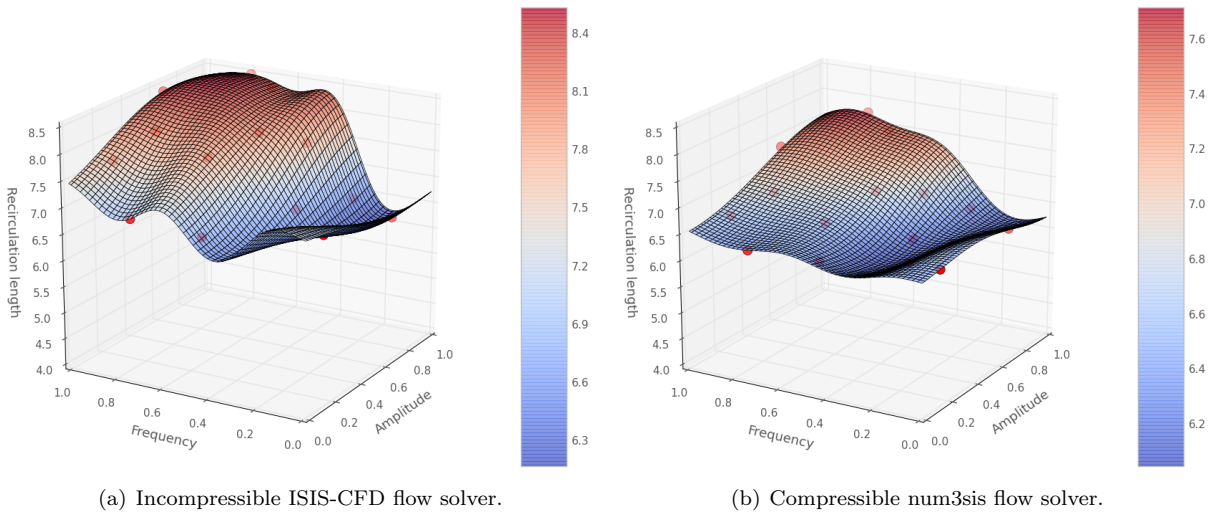
Figure 10. Influence of the flow solver on the bubble recirculation length.
