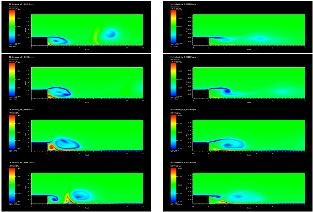
Figure 6. Comparison of the vorticity for k-\omega -ne-easm (left) and k-\omega -SST Menter (right) turbulence closure with 256 time steps by periods and the medium mesh. The current actuation point has an amplitude of 40.8m/s and a frequency of 113.333Hz . From top to bottom, the jet angular phase is \omega \approx 0 , \omega \approx \frac{\pi}{2} , \omega \approx \pi and \omega \approx \frac{3\pi}{2} .
