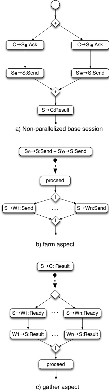
Figure 14: Managing data parallel computations
