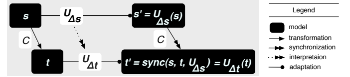
Fig. 3. Formalization of the incremental model synchronization.
