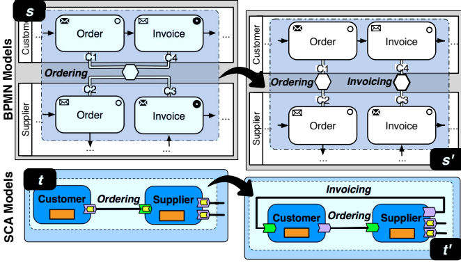
Fig. 2. BPMN and SCA model evolution use case.
