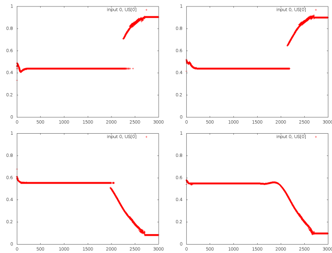
Figure 59: Splitted Amygdala predictions: the output selected based on the Decider Amygdala's predictions. Again, same problems than those shown in the figure 51
