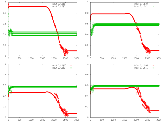
Figure 58: Decider Amygdala predictions, on red the predicted error for for the Cortex's Amygdala, on green, the predicted error for the Hippocampus' Amygdala. Generally the same problems than those shown in the figure 50
