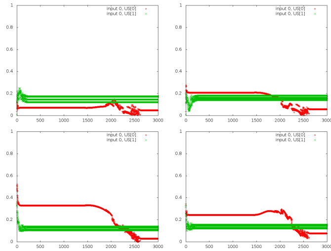
Figure 54: Decider Amygdala predictions, on red the predicted error for for the Cortex's Amygdala, on green, the predicted error for the Hippocampus' Amygdala. Similar problems than on figure 46
