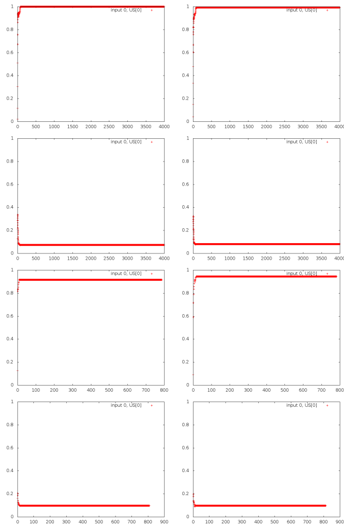
Figure 20: Outputs of Brain CHA for the double XOR, where A_2 , B_2 , AB_2 and Z_2 have 20% chance of appearing on each iteration. Again, no difference with the previous results). First row: A_1 and B_1 (US 1), second row: AB_1 and Z_1 (US 0), third row: A_2 and B_2 (US 1), last row: AB_2 and Z_2 (US 0)
