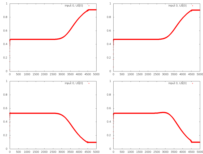
Figure 40: Predictions by the Cortex's Amygdala, very similar to figure 2. Top row: A and B (US 1), low row: AB and Z (US 0)
