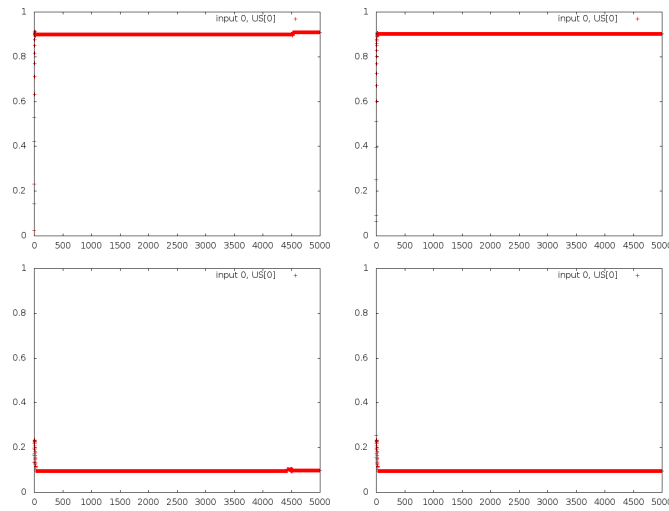
Figure 43: Splitted Amygdala predictions: the output selected based on the Decider Amygdala's predictions. The only difference is for A, where the output changes for the last few hundred iterations. Top row: A and B (US 1), low row: AB and Z (US 0)
