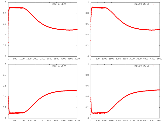
Figure 37: Outputs of Brain CHA for the simple XOR, with a forgetting rate of 0.00008 Top row: A and B (US 1), low row: AB and Z (US 0)
