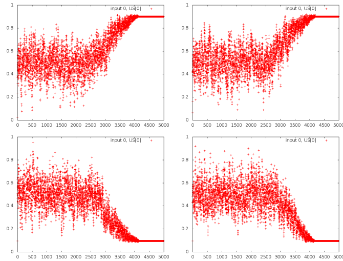
Figure 9: Outputs of Brain CA for the simple XOR, with the inputs randomized. The randomization changes the flatline state by random noise, until the Cortex's activity is strong enough to generate a convergence.
