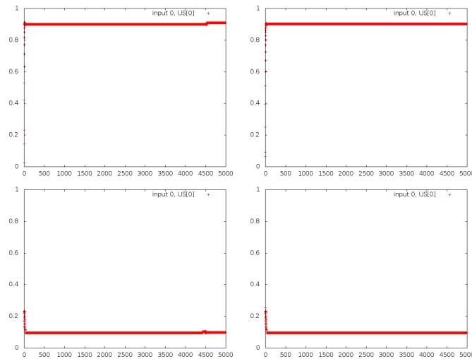
Figure 43: Splitted Amygdala predictions: the output selected based on the Decider Amygdala's predictions. The only difference is for A, where the output changes for the last few hundred iterations. Top row: A and B (US 1), low row: AB and Z (US 0)
