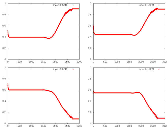
Figure 56: Predictions by the Cortex's Amygdala. Very similar to figure ?? as well. Top row: A and B (US 1), low row: AB and Z (US 0)
