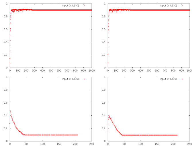
Figure 13: Outputs of Brain HA for the simple XOR, with the inputs disproportionate and randomized. It's basically a noisier version of fig. 7
