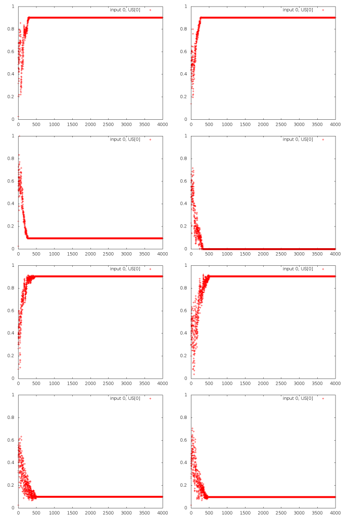
Figure 23: Outputs of Brain CA for the double XOR randomized, in a simulation that converged very fast. First row: A_1 and B_1 (US 1), second row: AB_1 and Z_1 (US 0), third row: A_2 and B_2 (US 1), last row: AB_2 and Z_2 (US 0)
