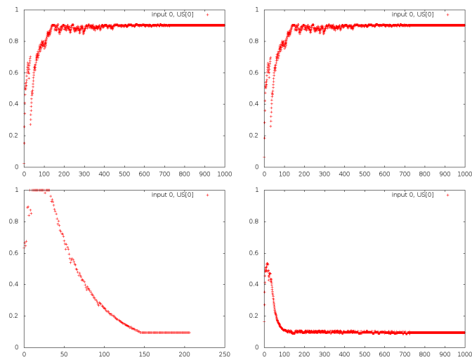
Figure 27: Brain without Hippocampus' outputs for the simple XOR with different probabilities on AB only Top row: A and B (US 1), low row: AB and Z (US 0)
