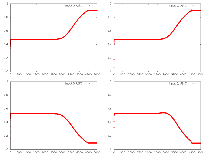
Figure 2: Outputs of Brain CA for the simple XOR showing the flatline until around the 2500th iteration and then the transition to the final convergence. Top row: A and B (US 1), low row: AB and Z (US 0)
