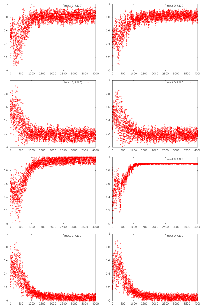
Figure 24: Outputs of Brain CA outputs for the double XOR randomized. These graphs aren't similar to any other, except for the one corresponding to B_2 . First row: A_1 and B_1 (US 1), second row: AB_1 and Z_1 (US 0), third row: A_2 and B_2 (US 1), last row: AB_2 and Z_2 (US 0)
