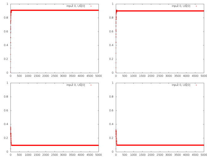
Figure 10: Outputs of Brain HA for the simple XOR, with the inputs randomized. This graph is practically identical to 3, the randomization doesn't affect the Hippocampus
