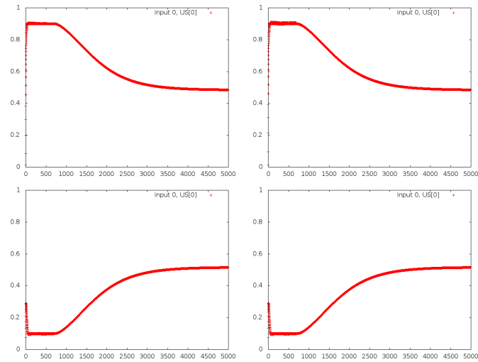
Figure 33: Outputs of Brain HA for the simple XOR, with a forgetting rate of 0.00008, which produces a faster return to predictions around 0.5, still useful. Top row: A and B (US 1), low row: AB and Z (US 0)
