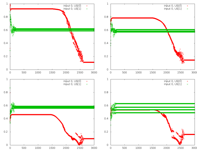
Figure 50: Decider Amygdala predictions, on red the predicted error for for the Cortex's Amygdala, on green, the predicted error for the Hippocampus' Amygdala. Again, large errors for A and B on red, but here the Decider Amygdala predicts worst behaviour than the real. Also, for Z the cycle of predicted values for the Hippocampus' Amygdala's error is wider. Top row: A and B (US 1), low row: AB and Z (US 0)
