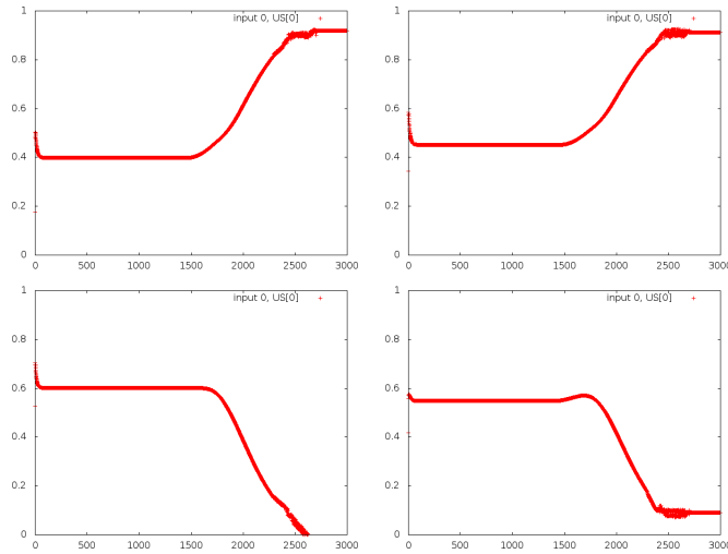
Figure 48: Predictions by the Cortex's Amygdala. Very similar to figure ??. Top row: A and B (US 1), low row: AB and Z (US 0)
