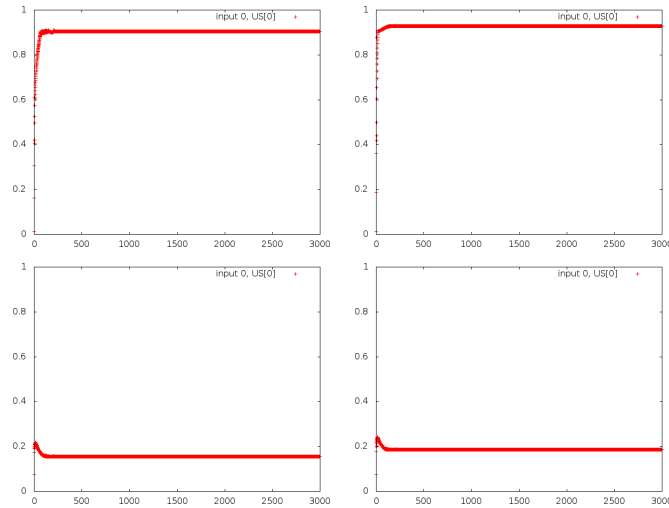
Figure 45: Predictions by the Hippocampus's Amygdala, similar to 3. Top row: A and B (US 1), low row: AB and Z (US 0)
