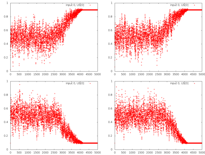
Figure 9: Outputs of Brain CA for the simple XOR, with the inputs randomized. The randomization changes the flatline state by random noise, until the Cortex's activity is strong enough to generate a convergence.
