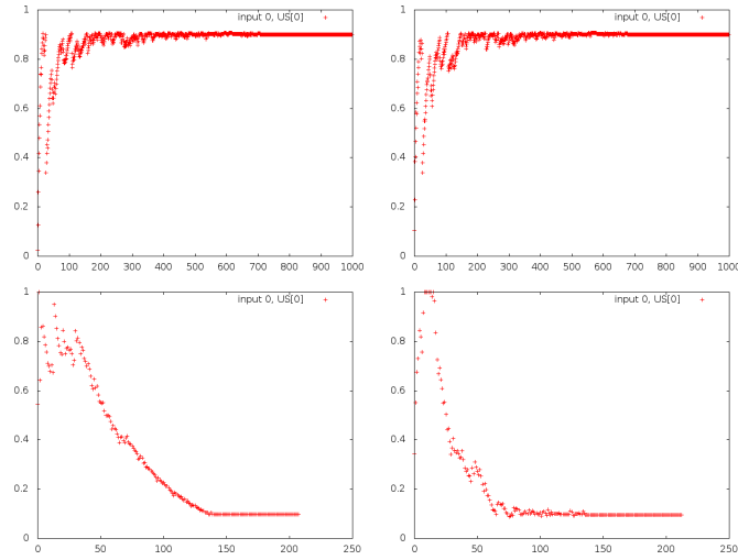
Figure 12: Outputs of Brain CA for the simple XOR, with the inputs disproportionate and randomized. This removes the noise shown in the figure 9, but the evolution to the convergence is noisier than in 6 for all four inputs.
