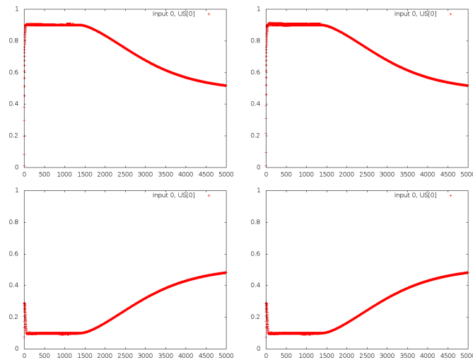
Figure 32: Outputs of Brain HA for the simple XOR, with a forgetting rate of 0.00005, which produces a gentle return to the flatline of the predictions. Top row: A and B (US 1), low row: AB and Z (US 0)
