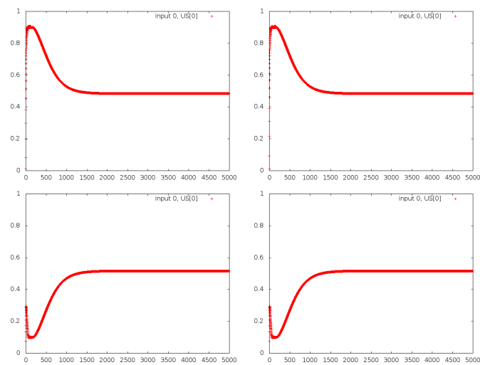
Figure 34: Outputs of Brain HA for the simple XOR, with a forgetting rate of 0.0002, which makes the predictions fall too fast, it could be said that there's no convergence. Top row: A and B (US 1), low row: AB and Z (US 0)
