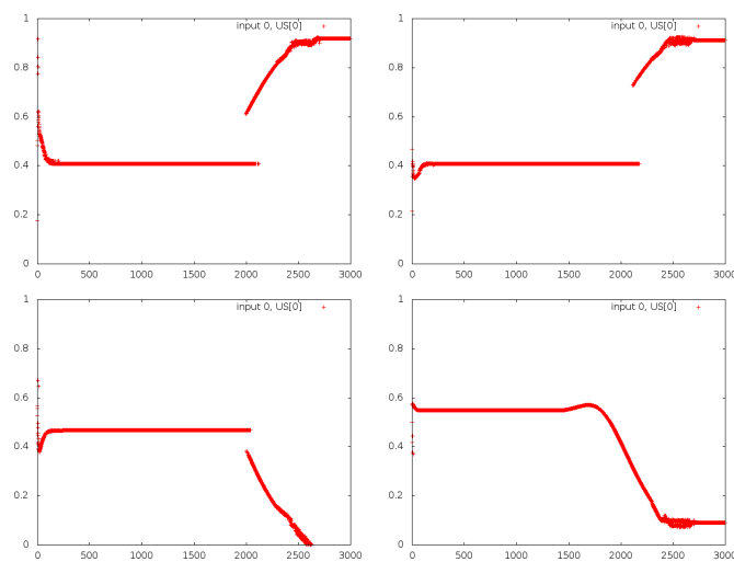
Figure 51: Splitted Amygdala predictions: the output selected based on the Decider Amygdala's predictions. Again, since the predictions are wrong, the selections are too, only this time it's picking the output from the Hippocampus instead of the Cortex. Top row: A and B (US 1), low row: AB and Z (US 0)
