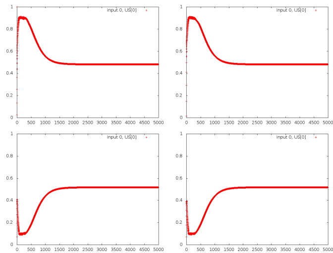
Figure 38: Outputs of Brain CHA for the simple XOR, with a forgetting rate of 0.0002 Top row: A and B (US 1), low row: AB and Z (US 0)
