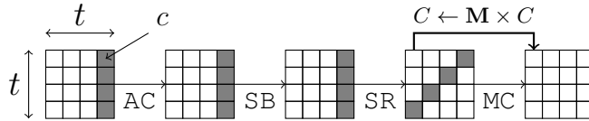
Figure 1: One round of the AES-like permutation instantiated with t = 4 .
