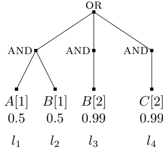
Figure 8: Example DNF tree for which the best schedule has larger cost than a non-linear strategy.
