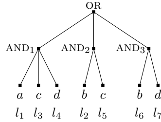
Figure 3: Example DNF tree.
