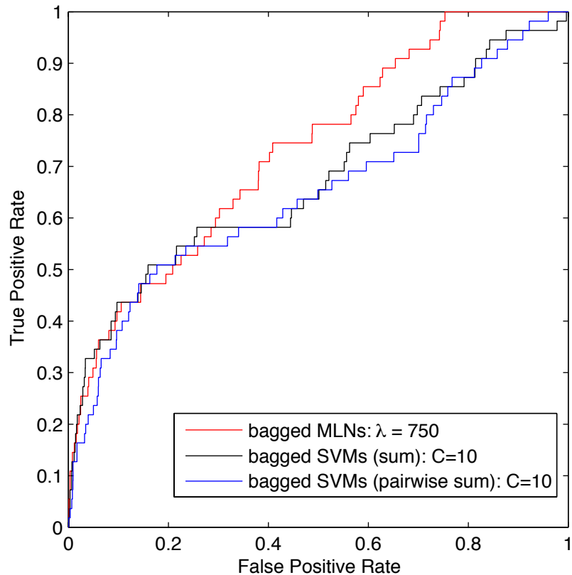
ROC curve
