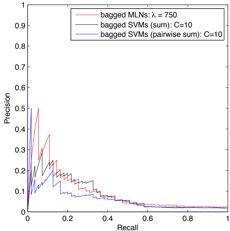
PR curve
