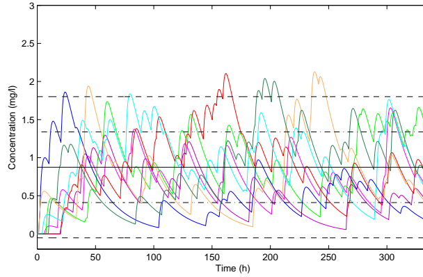
Figure 9: Eight sample paths of the concentration with Poisson distributed instant of intakes and uniformly distributed random doses, for the first 14 days. The black solid line is the limit concentration mean E(C^{rd}) , the dotted-dashed lines correspond to the confidence bands E(C^{rd}) \pm \sqrt{\text{Var}(C^{rd})} and the dashed lines to the confidence bands E(C^{rd}) \pm 2\sqrt{\text{Var}(C^{rd})} .
